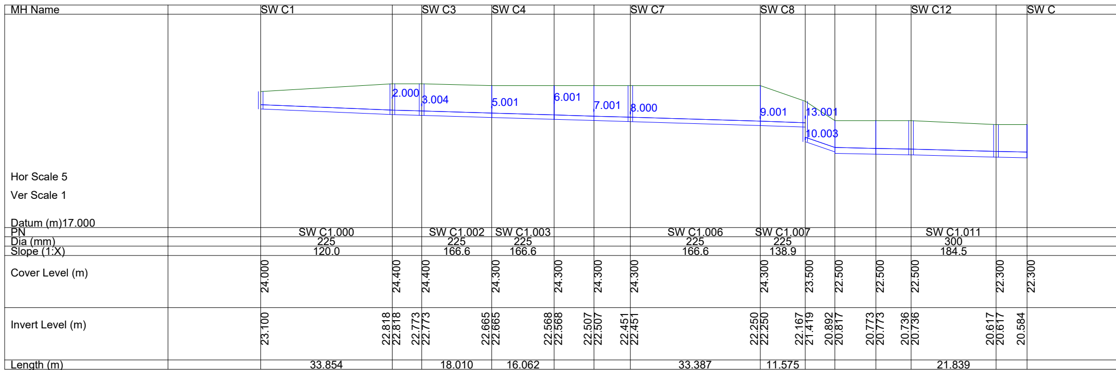
SURFACE WATER NETWORK: SW C1.000 - SW C1.012
