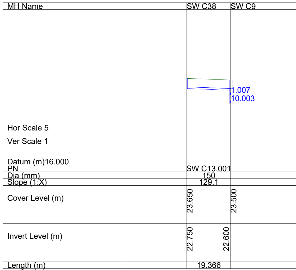
SURFACE WATER NETWORK: SW C1.000 - SW C1.012
