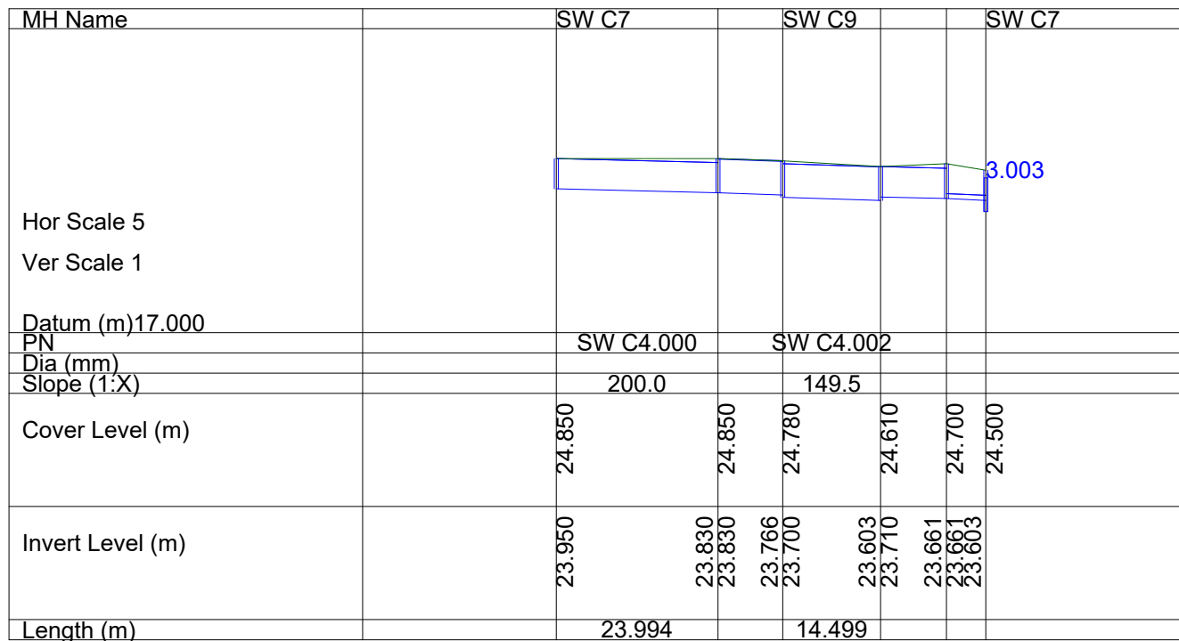
SURFACE WATER NETWORK: SW C1.000 - SW C1.012
