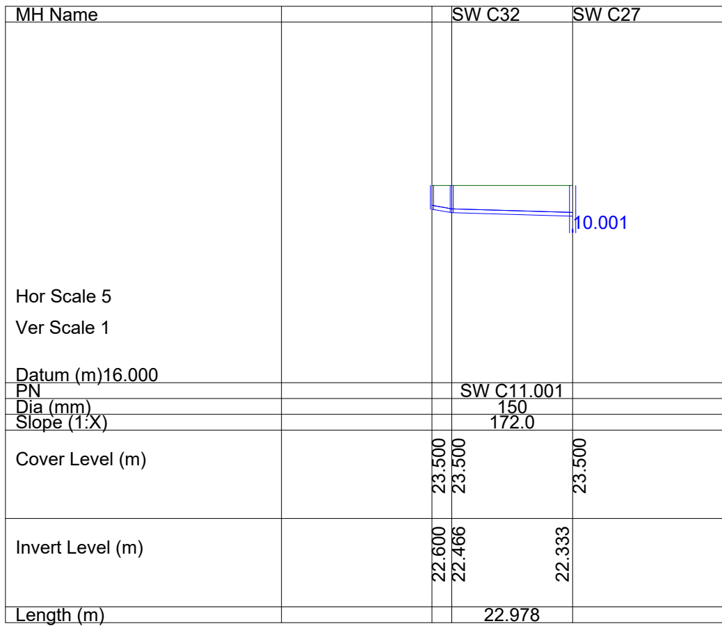
SURFACE WATER NETWORK: SW C1.000 - SW C1.012
